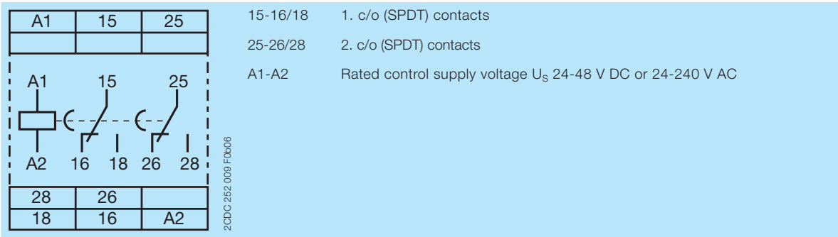
Connection diagram
