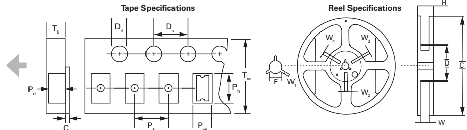
Dimensions for 0603, 0805, 1206, 1210, 1812 and 2920 size product (see table below)
