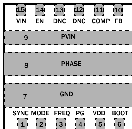
ISL85014 (15 LD 3.5mmx3.5mm TQFN) TOP VIEW
