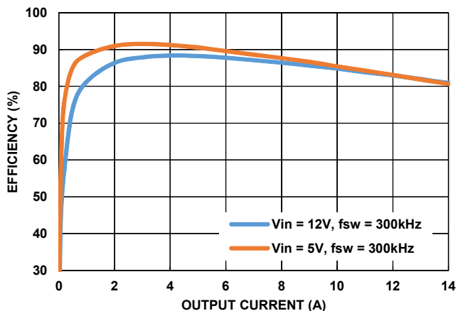
FIGURE 20. EFFICIENCY vs LOAD ( V_{OUT} = 1.0V , f_{SW} = 300kHz )
