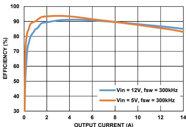
FIGURE 19. EFFICIENCY vs LOAD ( V_{OUT} = 1.2V , f_{SW} = 300kHz )
