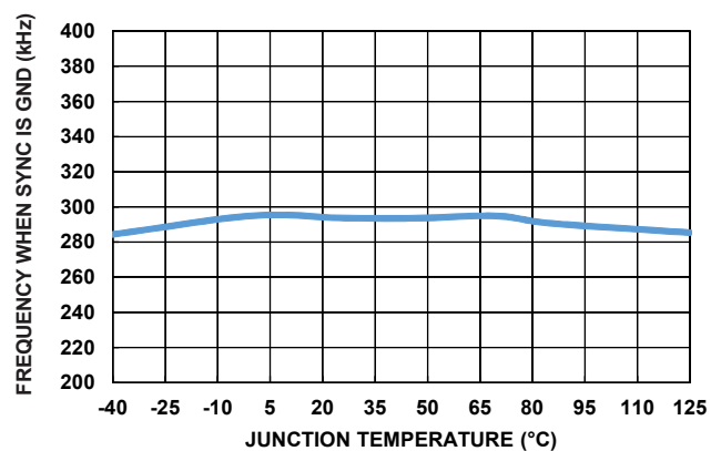
FIGURE 12. FREQUENCY (300kHz DEFAULT) vs TEMPERATURE
