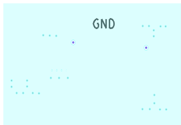
FIGURE 43. SOLID GND PLANE OF INNER LAYER 1
