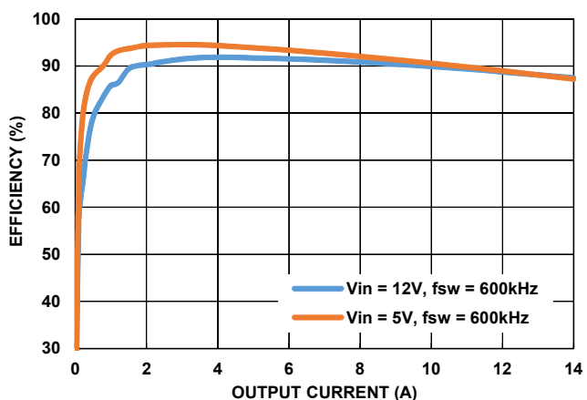
FIGURE 18. EFFICIENCY vs LOAD ( V_{OUT} = 1.8V , f_{SW} = 600kHz )
