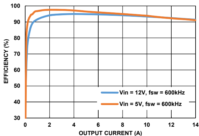
FIGURE 17. EFFICIENCY vs LOAD ( V_{OUT} = 3.3V , f_{SW} = 600kHz )
