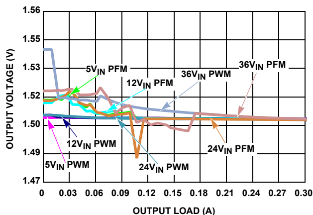
FIGURE 13. V_{OUT} REGULATION vs LOAD, PFM, V_{OUT} = 1.5\text{V}
