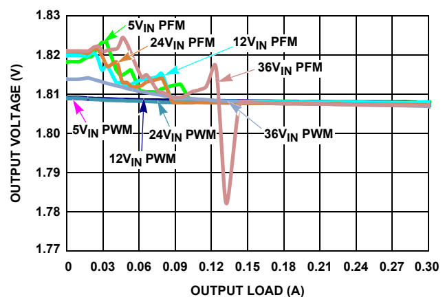
FIGURE 14. V_{OUT} REGULATION vs LOAD, PFM, V_{OUT} = 1.8\text{V}
